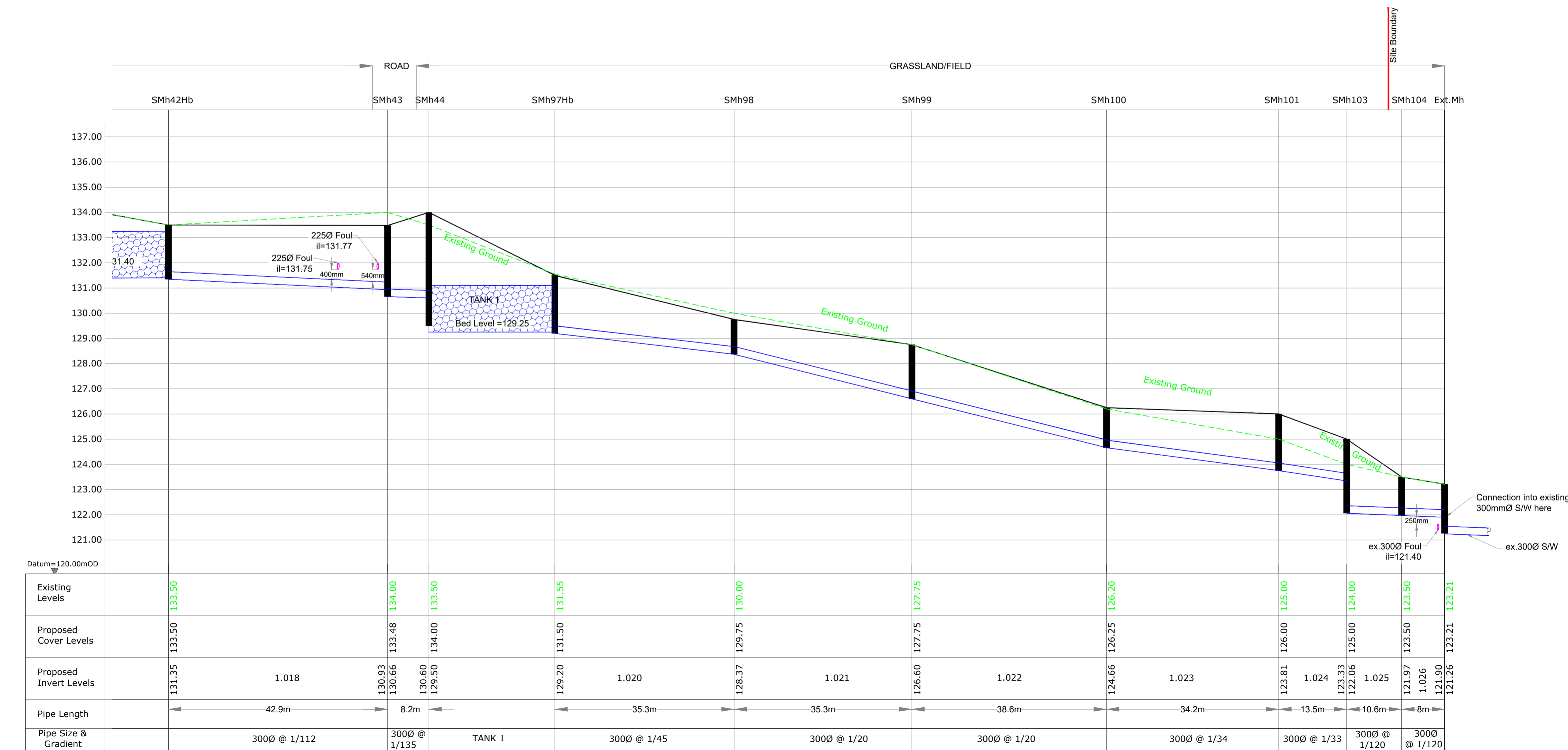
S/W Longitudinal Section SMh42Hb to Outfall
